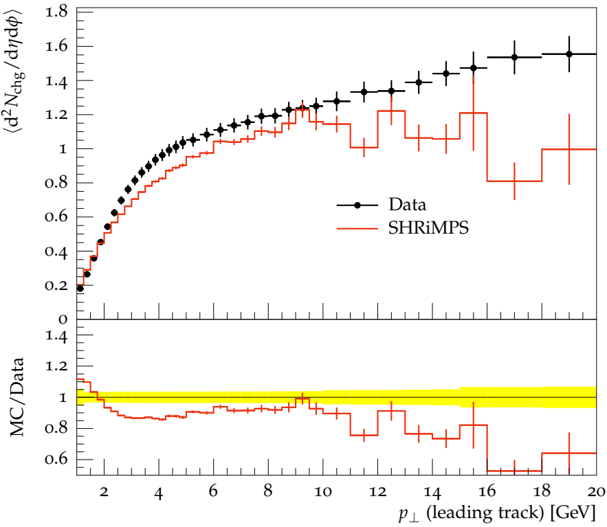
Away N_{\text{chg}} density vs. p_{\perp}^{\text{trk1}} , \sqrt{s} = 7 TeV
