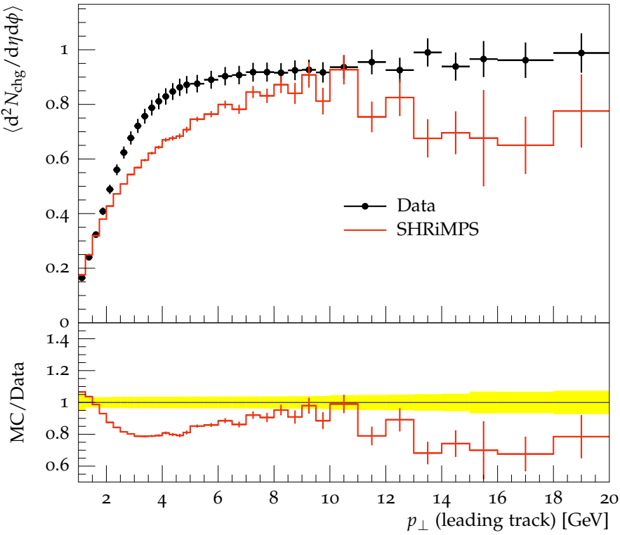
Transverse N_{\text{chg}} density vs. p_{\perp}^{\text{trk1}} , \sqrt{s} = 7 TeV
