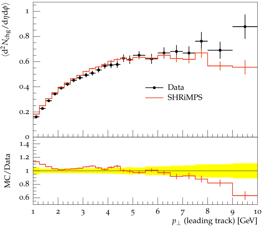
Away N_{\text{chg}} density vs. p_{\perp}^{\text{trk1}} , \sqrt{s} = 900 GeV
