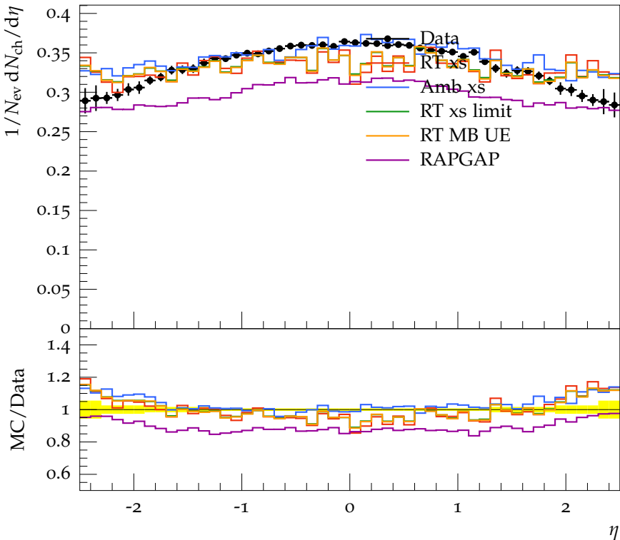
Charged particle \eta at 7 TeV, track p_{\perp} > 2500 MeV, for N_{\text{ch}} \geq 1
