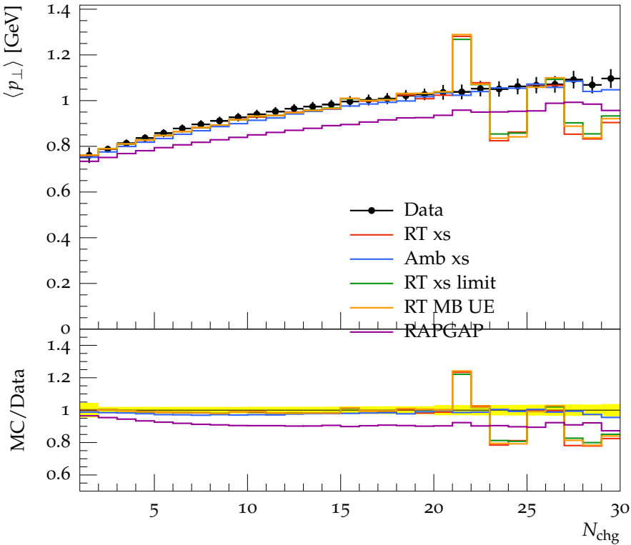
Transverse \langle p_{\perp} \rangle vs. N_{\text{chgr}} , \sqrt{s} = 7 TeV
