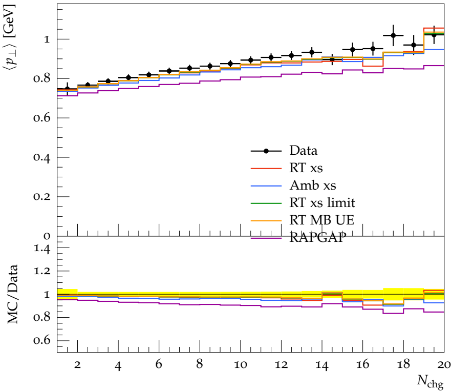
Transverse \langle p_{\perp} \rangle vs. N_{\text{chgr}} , \sqrt{s} = 900 GeV
