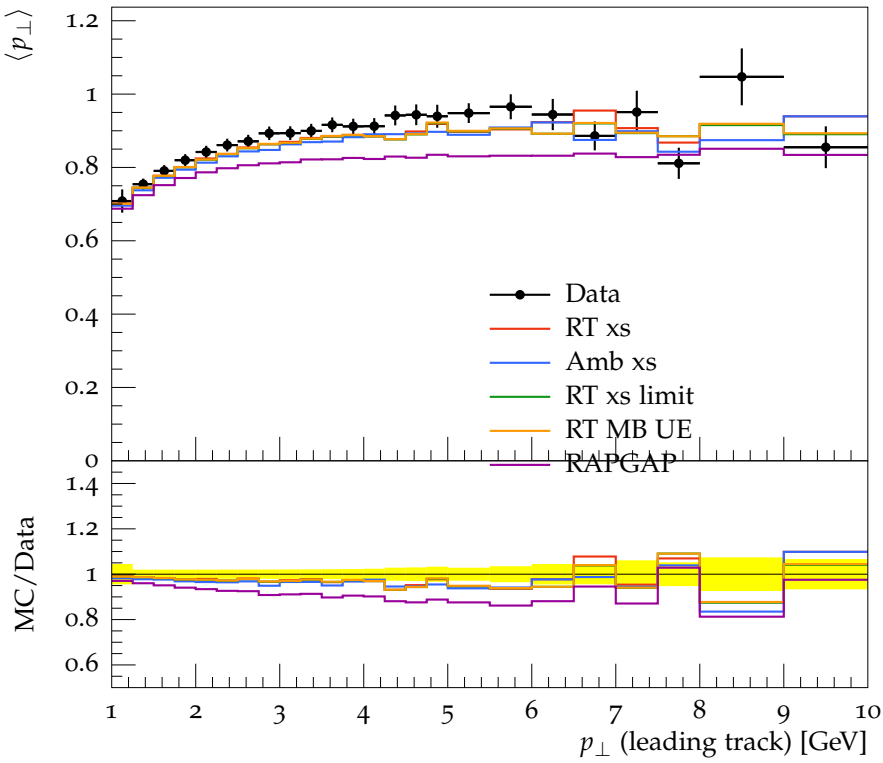
Transverse \langle p_{\perp} \rangle vs. p_{\perp}^{\text{trk1}} , \sqrt{s} = 900 GeV
