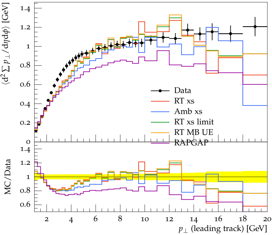
Transverse \Sigma p_{\perp} density vs. p_{\perp}^{\text{trk1}} , \sqrt{s} = 7 TeV
