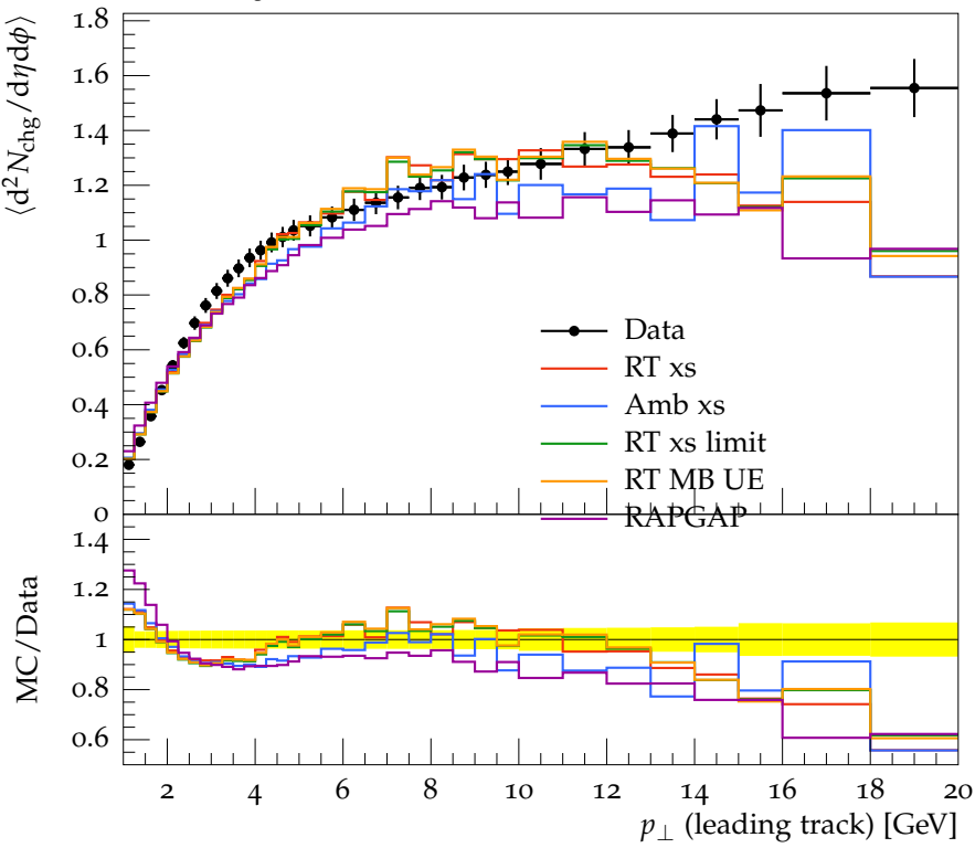
Away N_{\text{chg}} density vs. p_{\perp}^{\text{trk1}} , \sqrt{s} = 7 TeV
