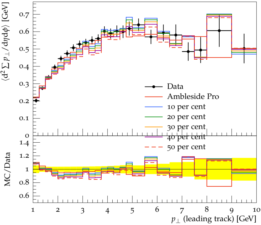
Transverse \Sigma p_{\perp} density vs. p_{\perp}^{\text{trk1}} , \sqrt{s} = 900 GeV, p_{\perp} > 100 MeV
