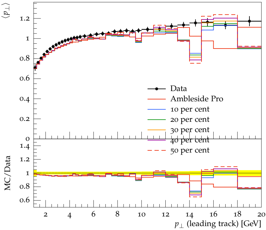
Transverse \langle p_{\perp} \rangle vs. p_{\perp}^{\text{trk1}} , \sqrt{s} = 7 TeV
