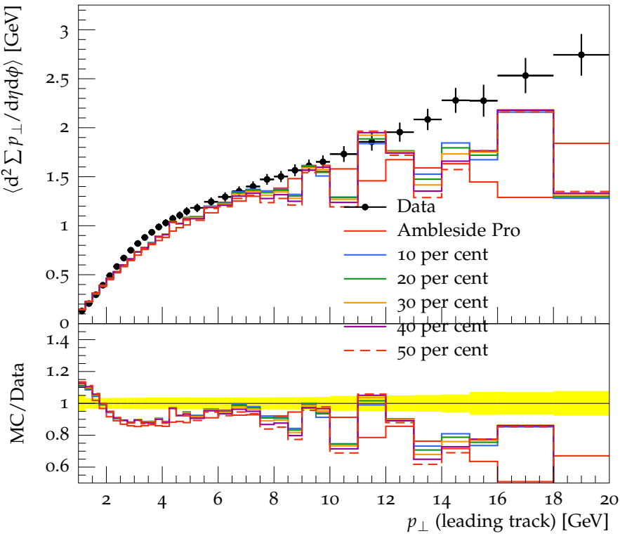
Away \Sigma p_{\perp} density vs. p_{\perp}^{\text{trk1}} , \sqrt{s} = 7 TeV
