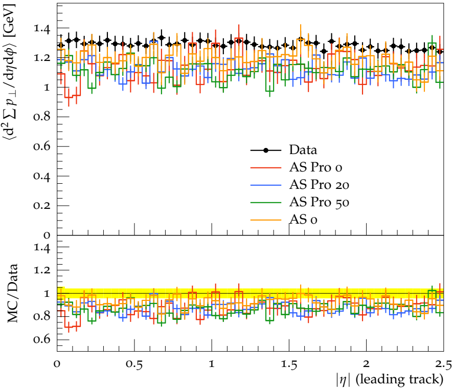
Transverse \Sigma p_{\perp} density vs. |\eta^{\text{trk1}}| , \sqrt{s} = 7 TeV, p_{\perp} > 100 MeV
