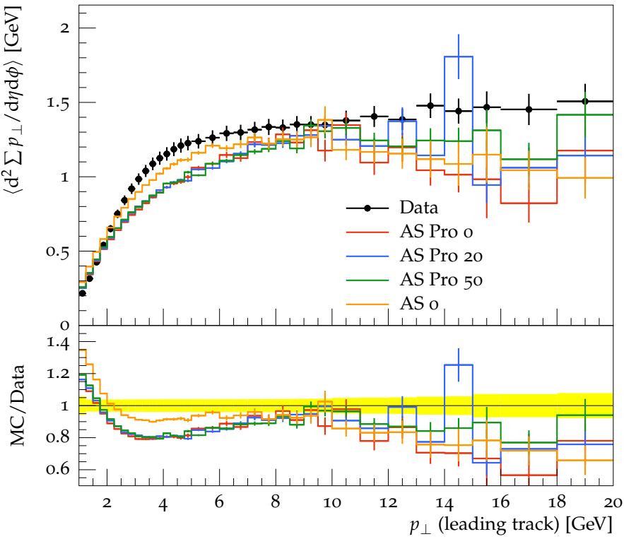
Transverse \Sigma p_{\perp} density vs. p_{\perp}^{\text{trk1}} , \sqrt{s} = 7 TeV, p_{\perp} > 100 MeV
