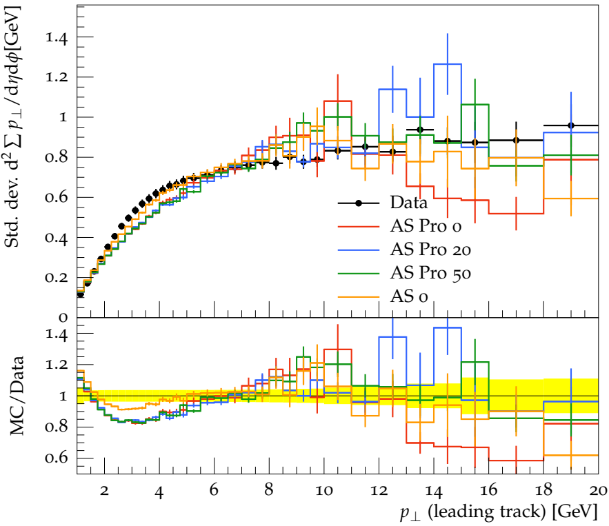
Std. dev. Transverse \Sigma p_{\perp} density vs. p_{\perp}^{\text{trk1}} , \sqrt{s} = 7 TeV
