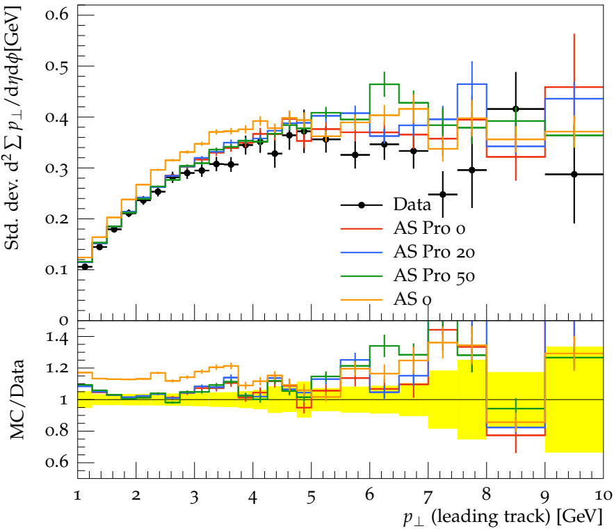
Std. dev. Transverse \Sigma p_{\perp} density vs. p_{\perp}^{\text{trk1}} , \sqrt{s} = 900 GeV
