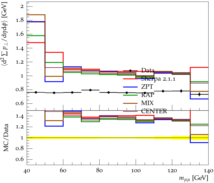
Towards + transverse \Sigma p_{\perp} density vs m_{\mu\mu} , p_{\perp}^{\mu\mu} < 5 GeV
