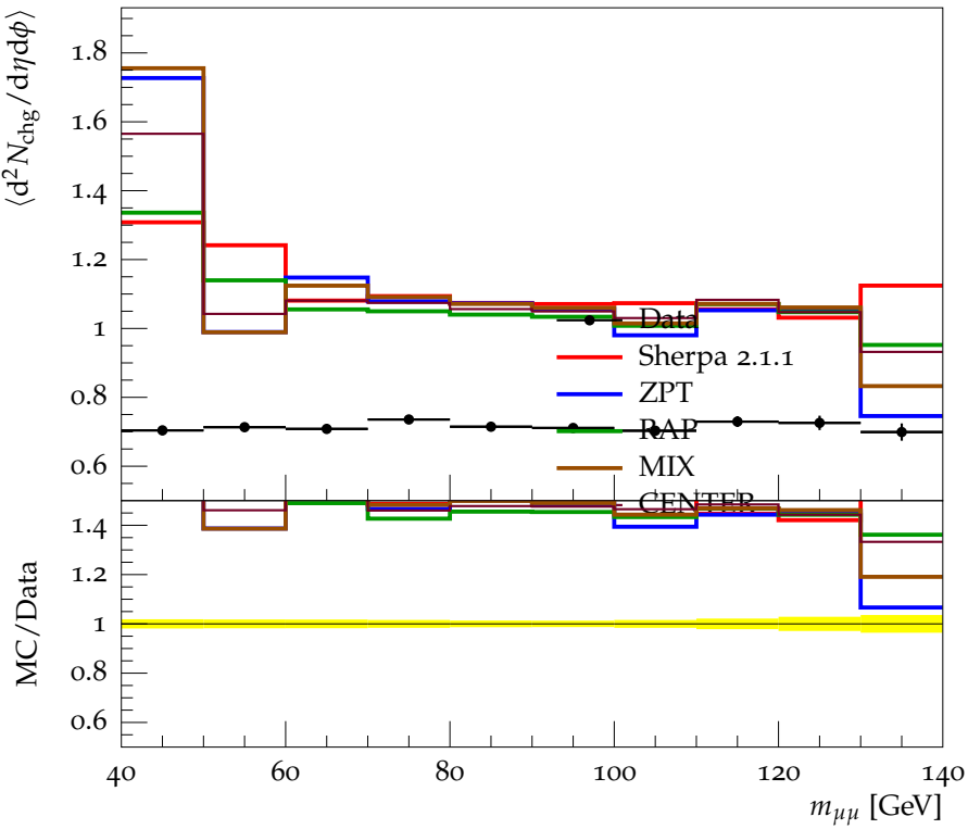
Towards + transverse N_{\text{chg}} density vs m_{\mu\mu} , p_{\perp}^{\mu\mu} < 5 GeV
