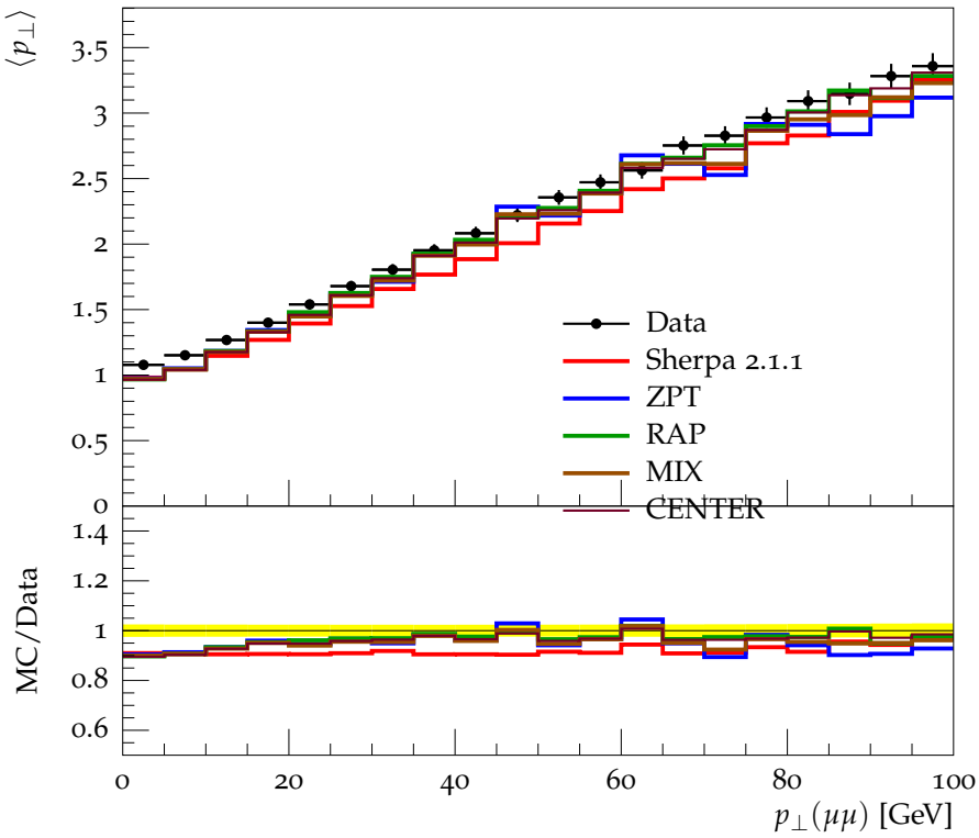
Away \langle p_{\perp} \rangle vs p_{\perp}^{\mu\mu}
