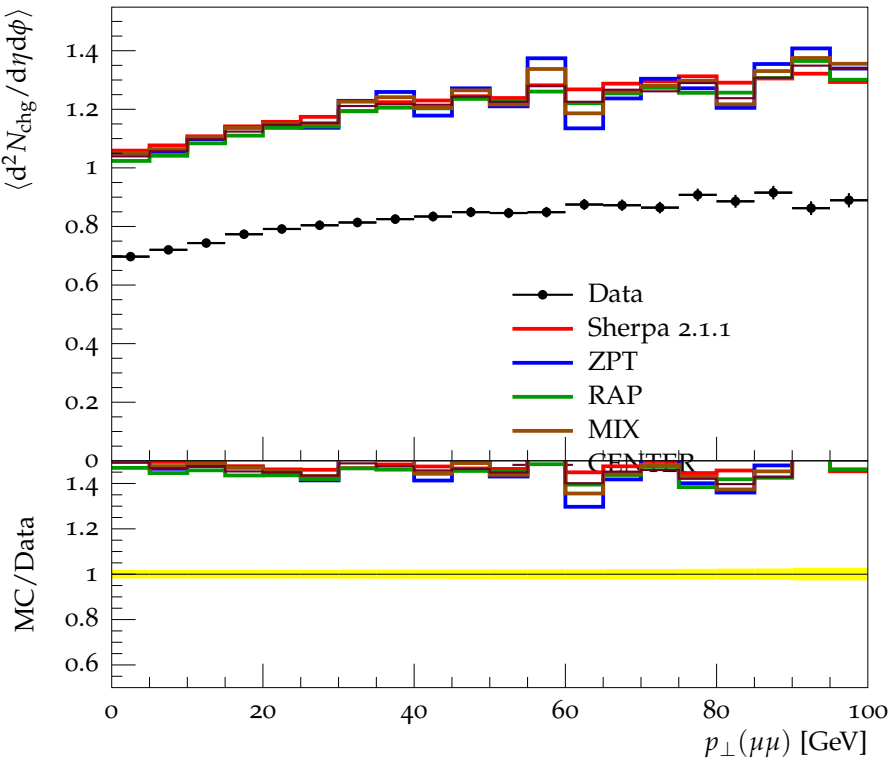
Toward N_{\text{chg}} density vs p_{\perp}^{\mu\mu}
