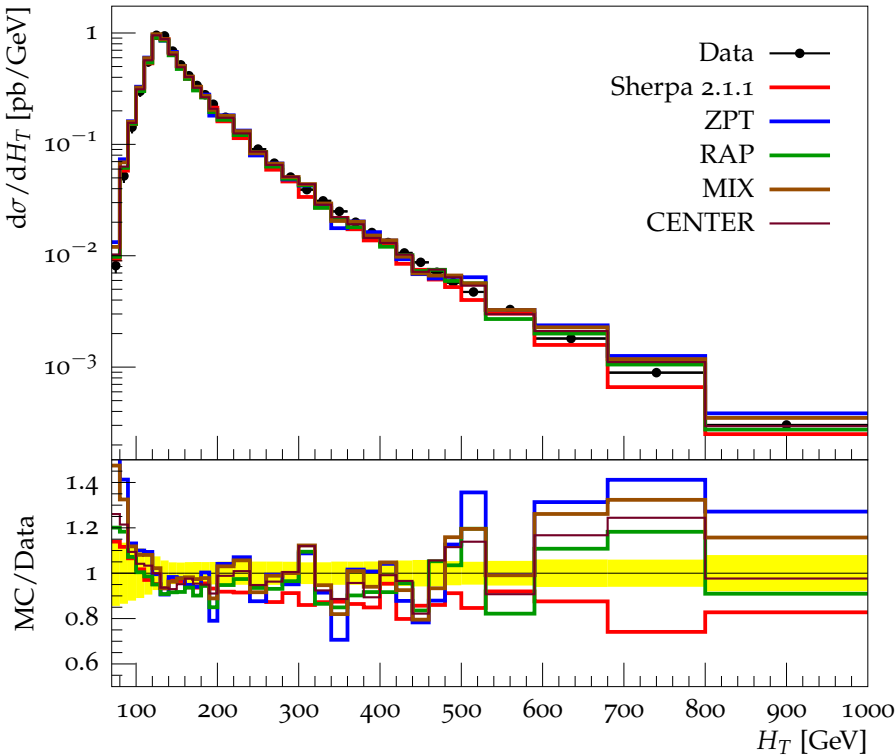
Scalar p_{\perp} sum of leptons and jets
