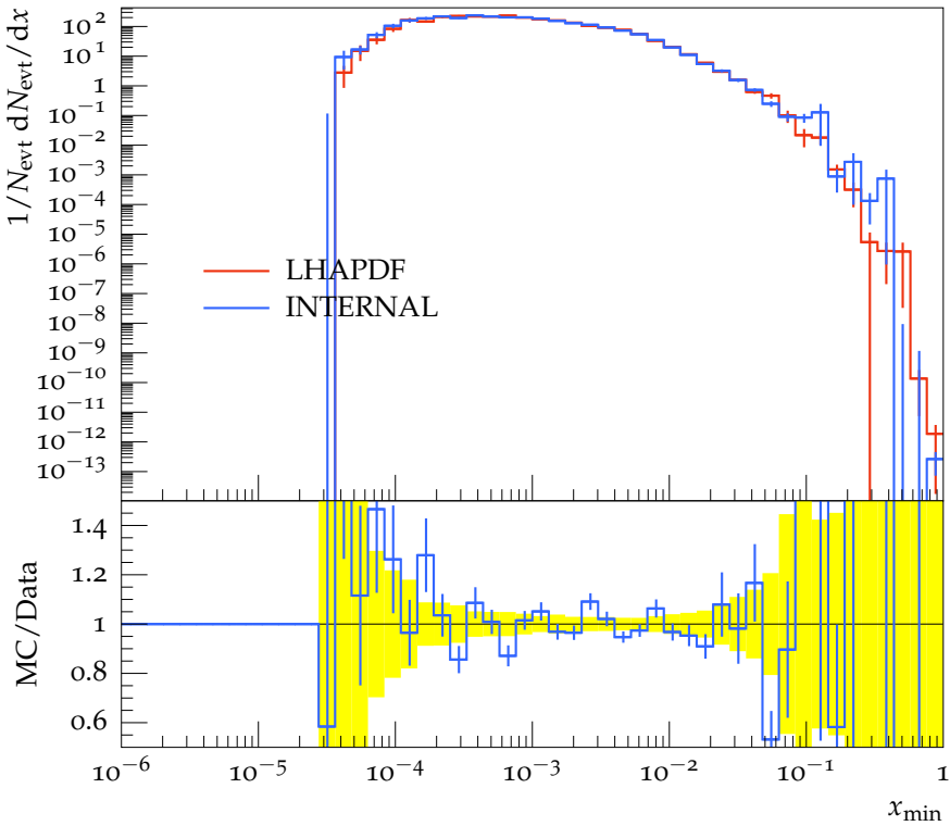
PDF sampling x_{\min} value distribution
