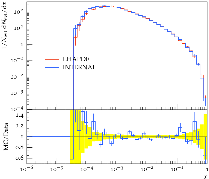
PDF sampling x value distribution
