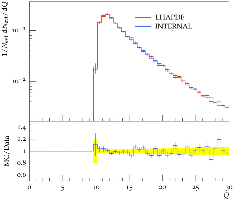
PDF sampling Q value distribution
