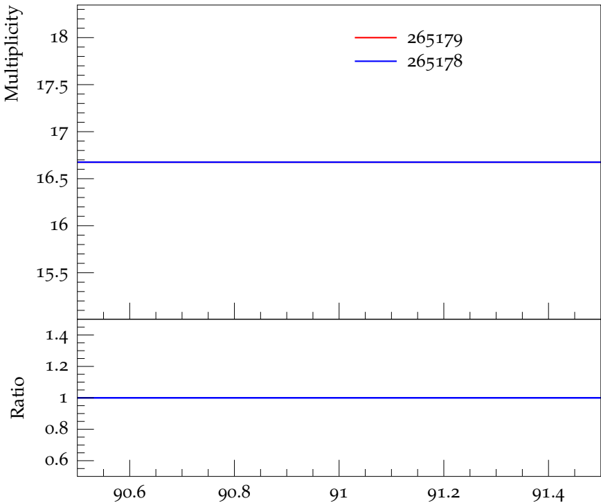
Mean \pi^+ multiplicity
